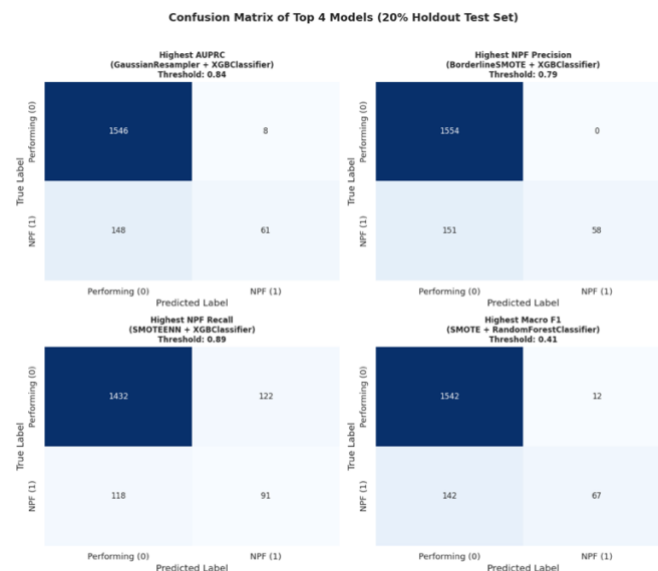
Figure 2. Confusion Matrices of the Four Selected Configurations
