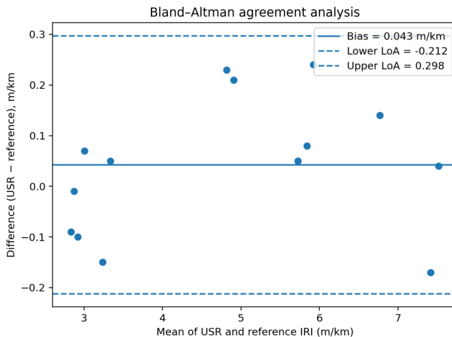
Figure 2. Bland-Altman agreement analysis for the 15 paired observations.
