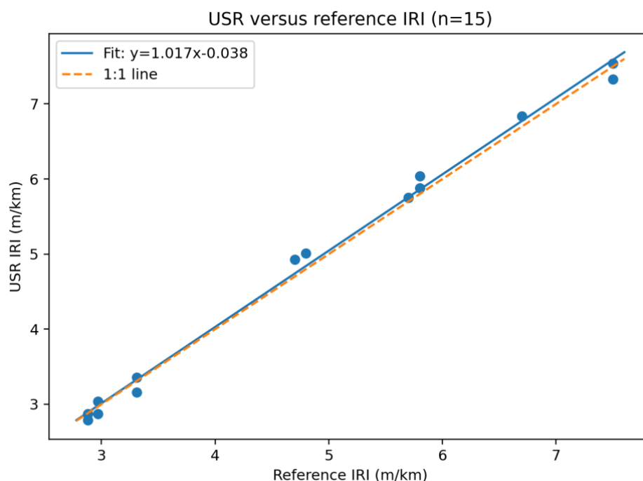
Figure 1. USR versus reference IRI with fitted regression and 1:1 line.
