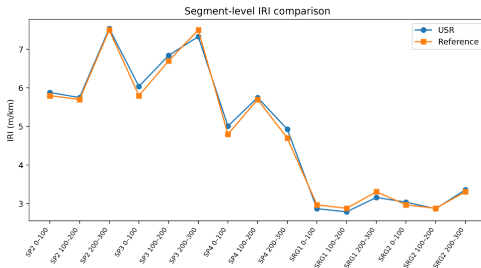
Figure 3. Segment-level comparison of USR and reference IRI.
