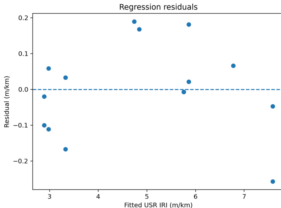
Figure 4. Regression residuals.
